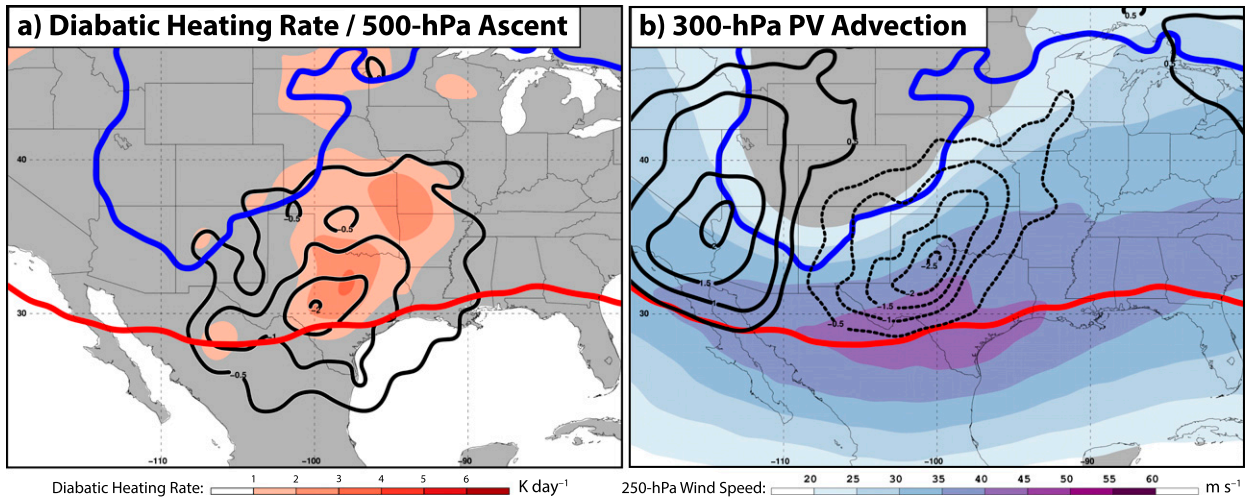
FIG. 6. (a) The 500-hPa diabatic heating rate (shaded according to the legend in \text{K day}^{-1} ), 500-hPa ascent (black lines every -0.5 \text{ dPa}^{-1} ), and the position of the 2-PVU contour within the 320–325-K and the 345–350-K layer is indicated by the thick blue and red line, respectively, 24-h prior to a polar dominant jet superposition. (b) As in (a), but with 250-hPa wind speed (shaded according to the legend in \text{m s}^{-1} ), and 300-hPa PV advection by the three-dimensional divergent circulation (black contours every 0.5 \times 10^{-5} \text{ PVU s}^{-1} , solid when positive and dashed when negative).
